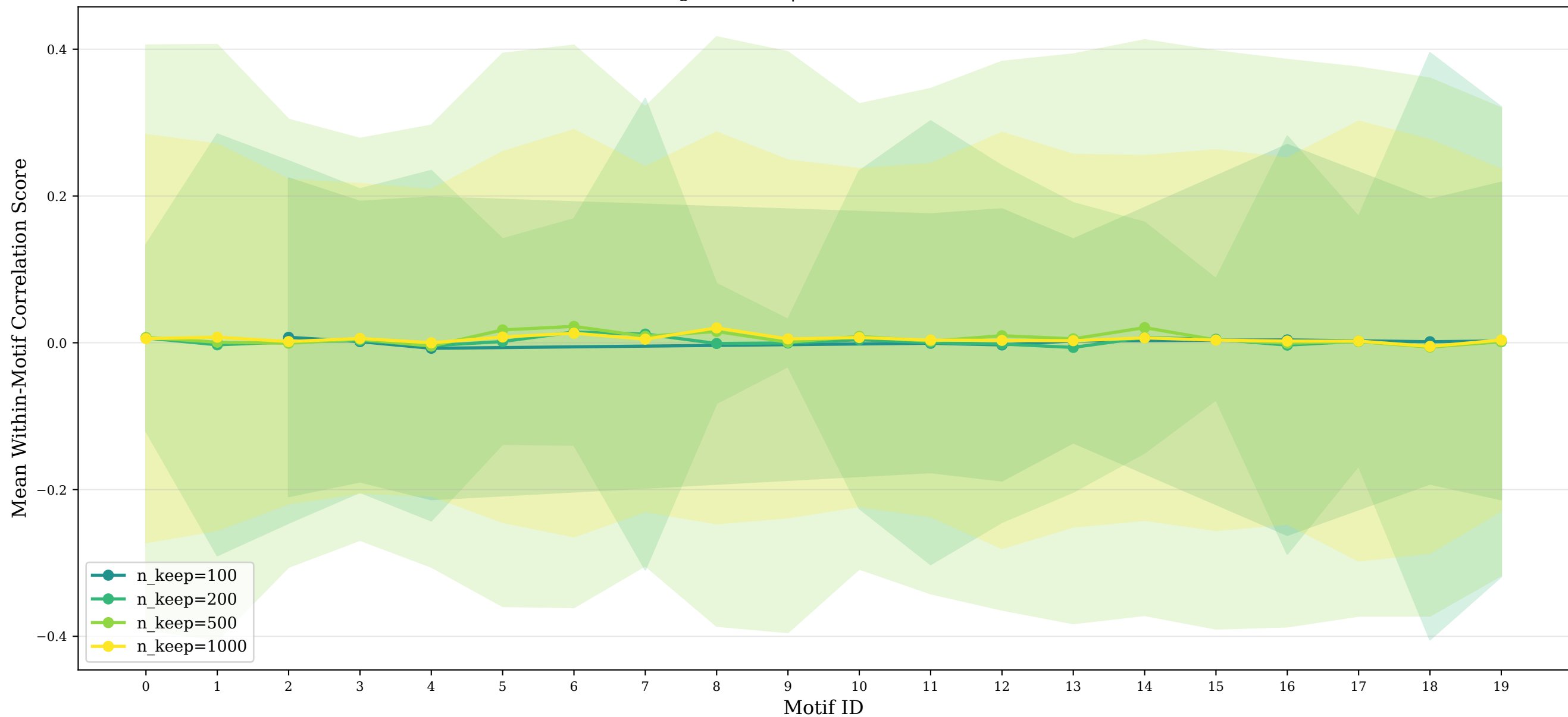
Correlation Score per Motif at Different Downsampling Levels (min_length=5) sigma: (1, 1) | volume: (0.03, 0.9)
